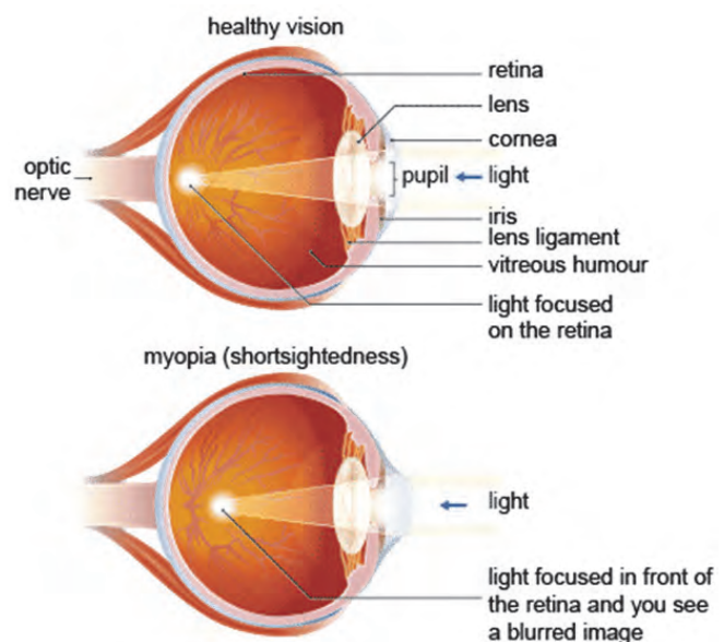
Figure 2-36: Short sightedness.
